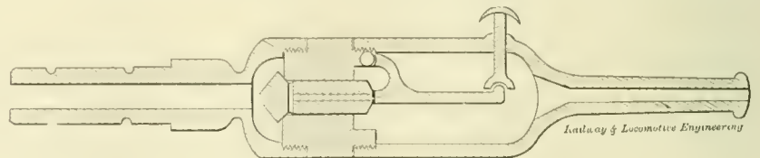
AN IMPROVED AIR NOZZLE VALVE.
